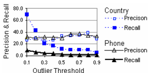
Figure 3: Performance of modified Lapis with outlier threshold expressed as a fraction of MAXDIST to centroid.
